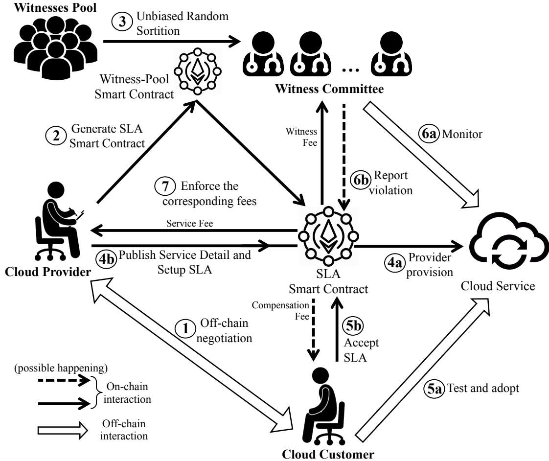
Figure 1: System Overview for Cloud SLA Enforcement
